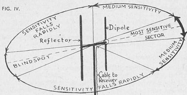
Sensitivity diagram of a typical H-shaped aerial
