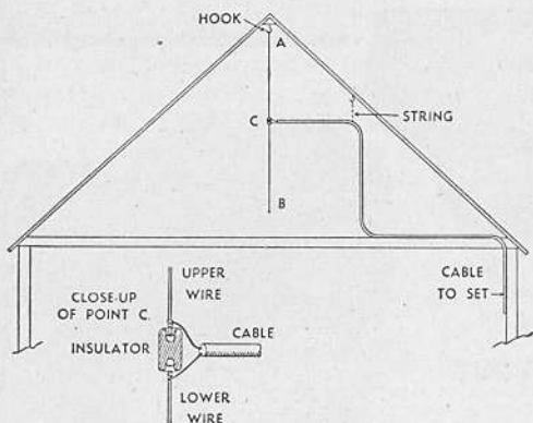
FIG. V. A Simple Wire Dipole Aerial in the Loft The length A—B is to be as in the Table.
