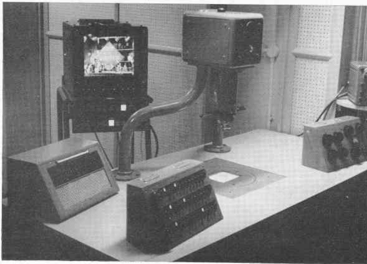
Inlay/Overlay equipment for the production of special effects. An example of its use is illustrated. A portion of the picture from one camera is blacked out by placing a diamond shaped mask over the raster from a flying spot scanner in the centre of the control desk. This space is filled with a caption from a second camera.
