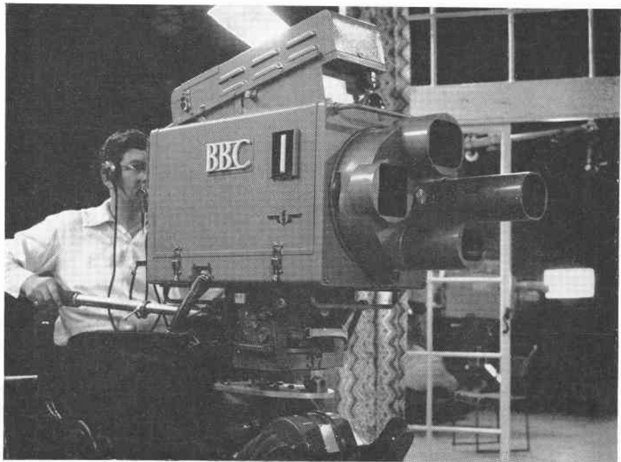
One type of modern camera showing the rotating lens turret, fitted with four lenses of different focal lengths, and an electronic viewfinder.
